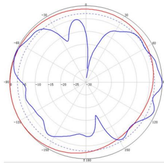
617~960MHz Typical pattern:
