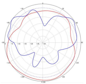
3300~6000MHz Typical pattern:
